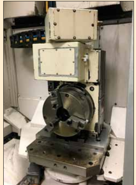
OKUMA # MA-400HA "5-AXIS" CNC HORIZONTAL MACHINING CENTER W/ TSUDAKOMA 5TH-AXIS ROTARY TABLES
