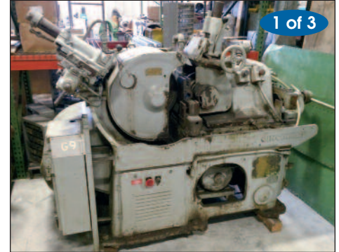
CINCINNATI # 2 CENTERLESS GRINDER
